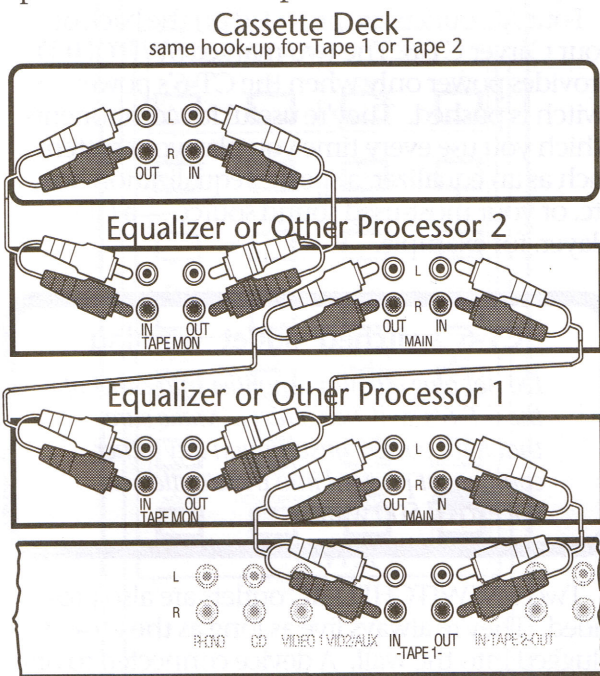
CT-6 Tuner/Preamplifier "alternative" hook-up would return MAIN OUTPUT of Processor 1 to CT-6's VIDEO 1 or VIDEO 2
